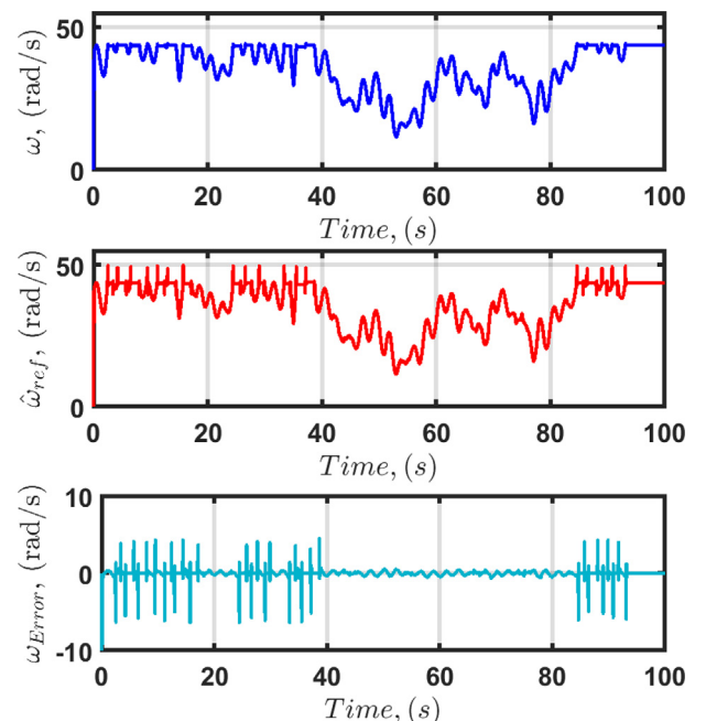
Fig. 9. Scenario 2. Speed tracking performance with the proposed HOODO-based LQR for r = 2 .
