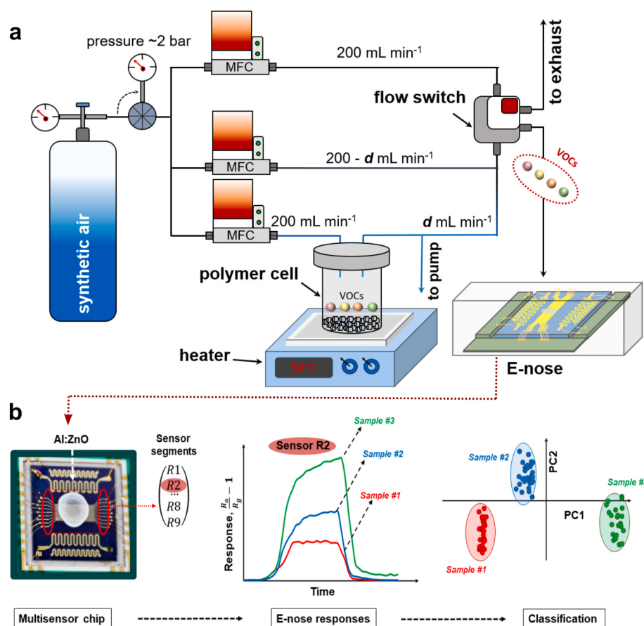
Fig. 1. Design of a setup for estimating the food plastic odors using an Al-doped ZnO-based electronic nose: (a) scheme of a gas-analytical system; (b) illustration of the sensor chip operation when exposed to organic impurities from the polymer granules with further classification of the responses by pattern recognition methods.
