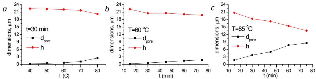
Fig. 5. Dependences of pores diameters and thicknesses of TMs: (a) on etching temperature at etching time 30 min; (b) dependence of pores diameters on etching time at temperatures 60 °C and (c) 85 °C.
