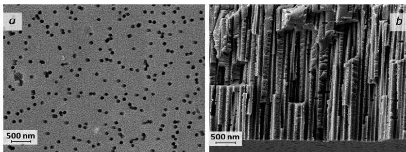
Fig. 2. (a) Example of SEM images of the surface and (b) cross-section of the PET template.
