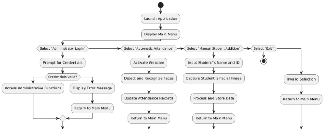
Figure 1 User flow diagram for student attendance management system
