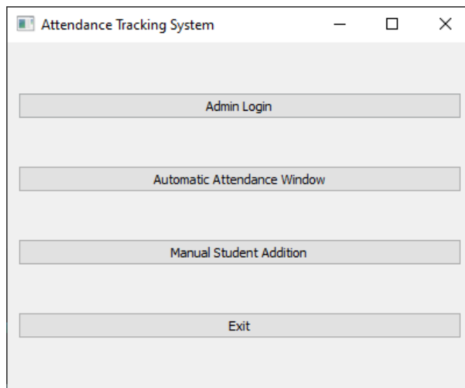
Figure 2 Main Window
