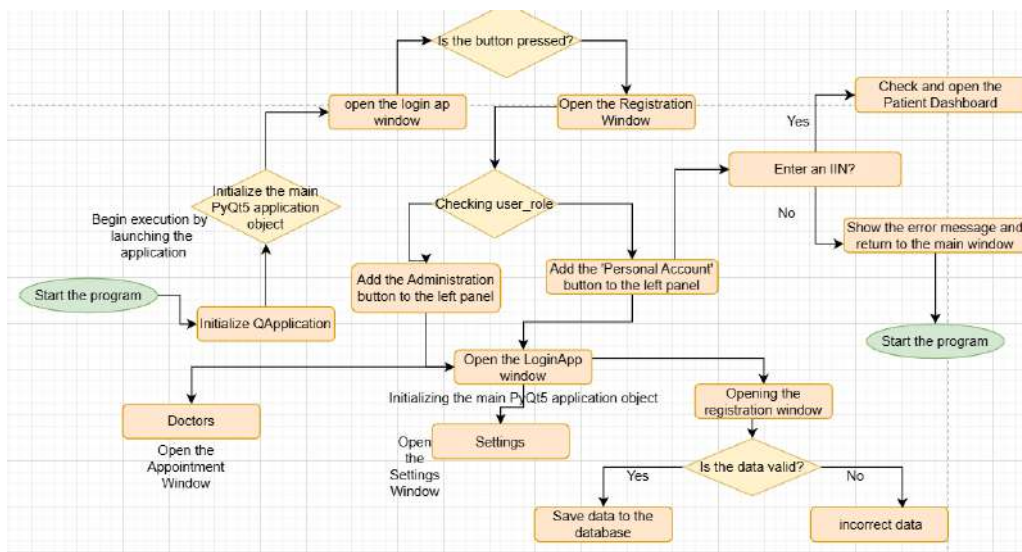
Figure 2. User authentication and registration algorithm
