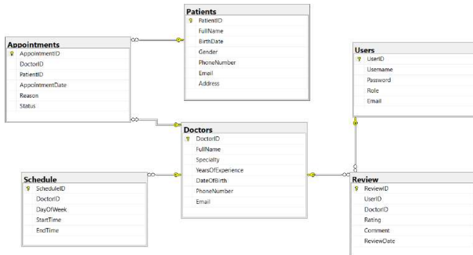
Figure 1. Creating a project database diagram
