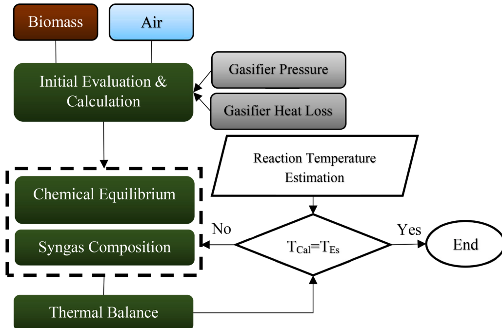
Fig. 2. Gasification thermodynamic analyses process flowchart.
