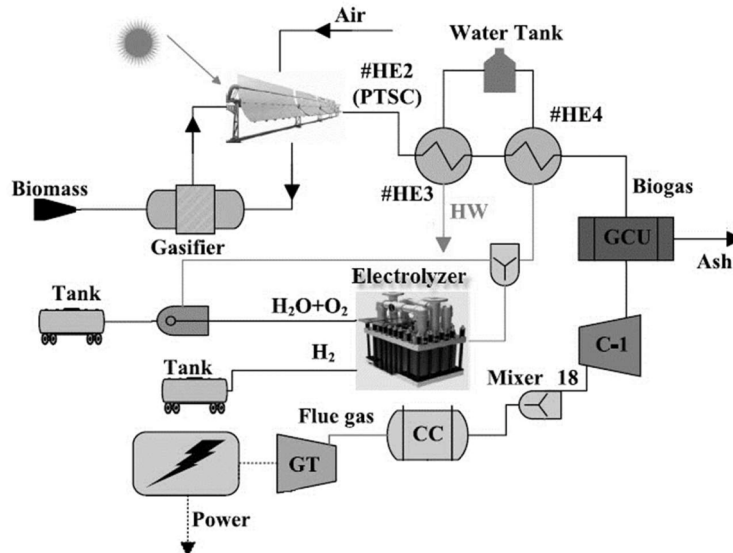
Fig. 1. Hybrid system scheme.
