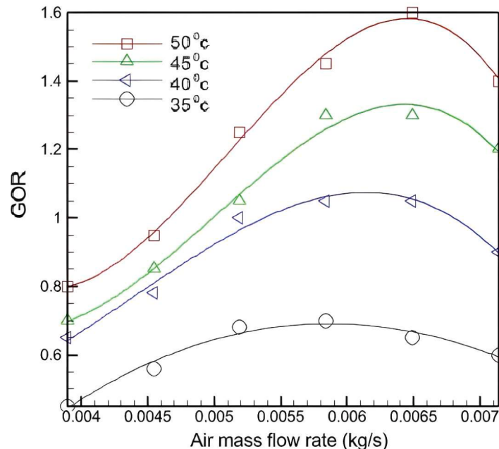
Fig. 9. Variation in GOR with \dot{m}_a .
