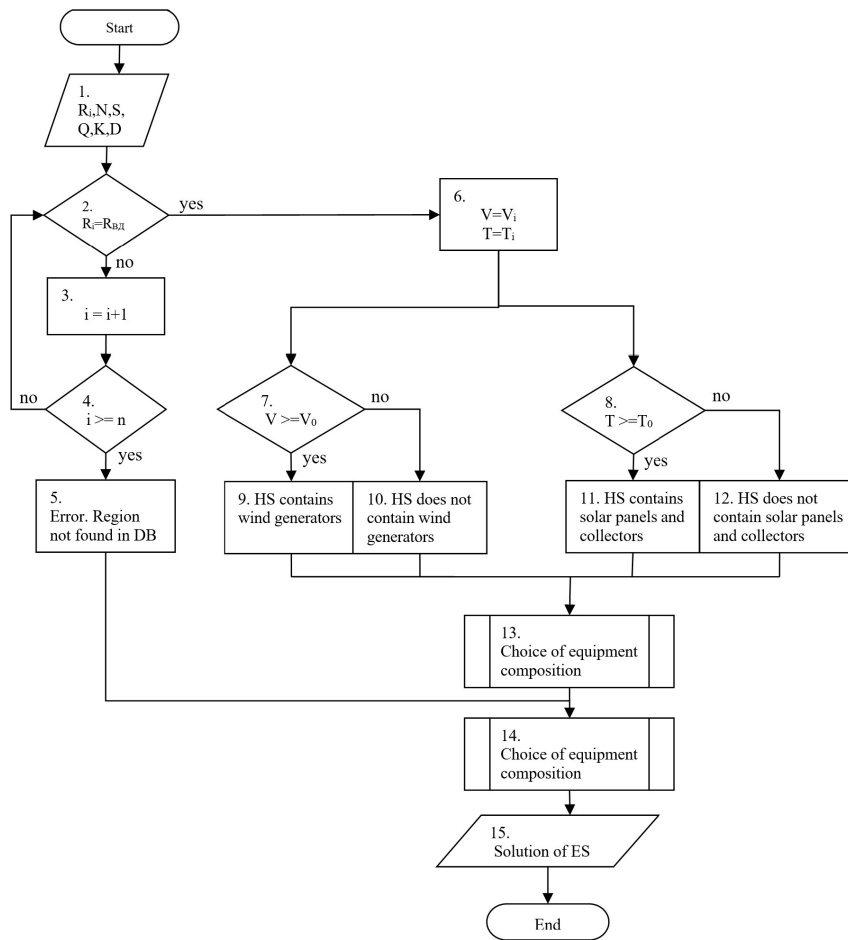
FIGURE 2 – ES work algorithm
