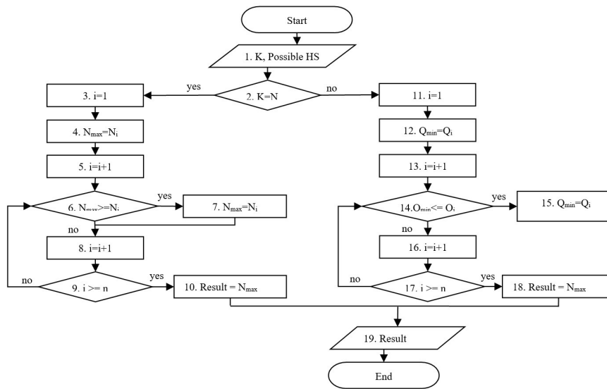
FIGURE 4 – The algorithm for finding the optimal solution
