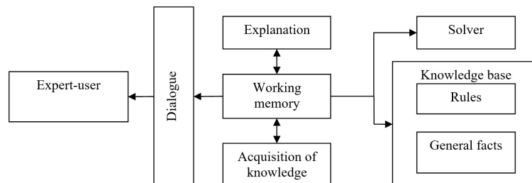
FIGURE 1 – The scheme of the generalized expert
