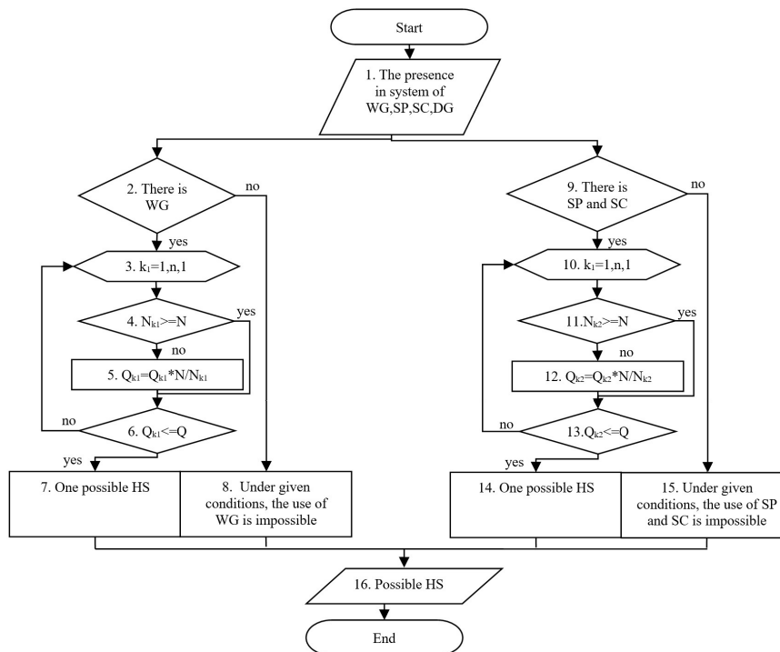
FIGURE 3 – Equipment search algorithm
