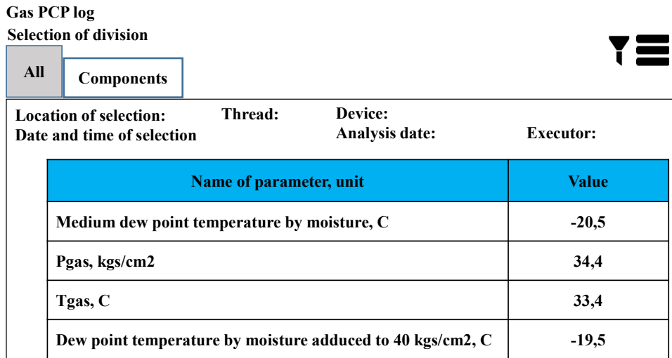
Fig. 2. An example of the interface of the “PChPs of Gas” function
