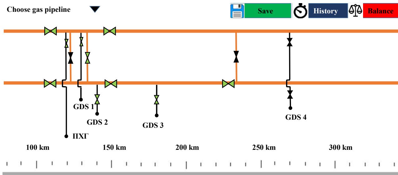
Fig. 3. An example of the “Gas Pipeline Section Selection” interface of the “Gas Balance and Metering” function
