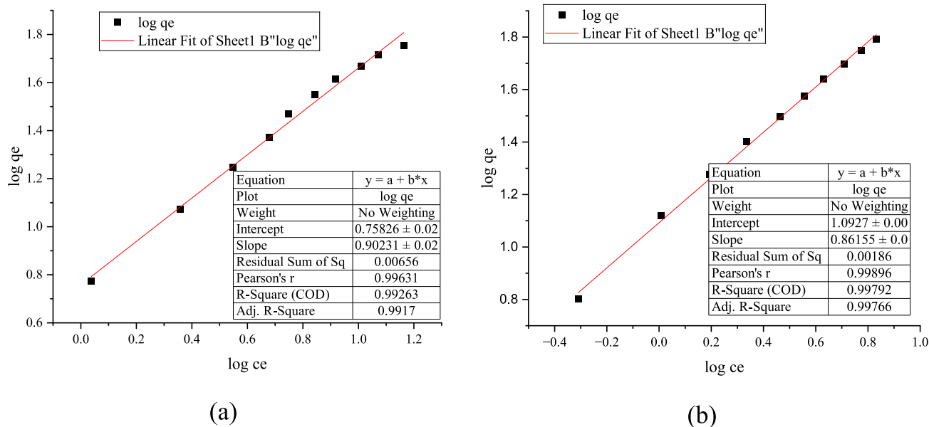
Fig. 4. Freundlich adsorption isotherm (a) without biofilm (b) with biofilm.
