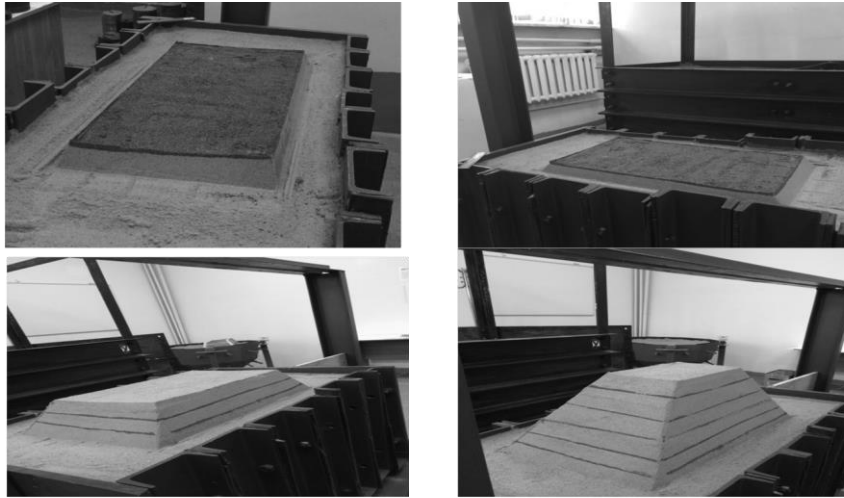
Figure 4. Layered laying of a dam model without reinforcement.
