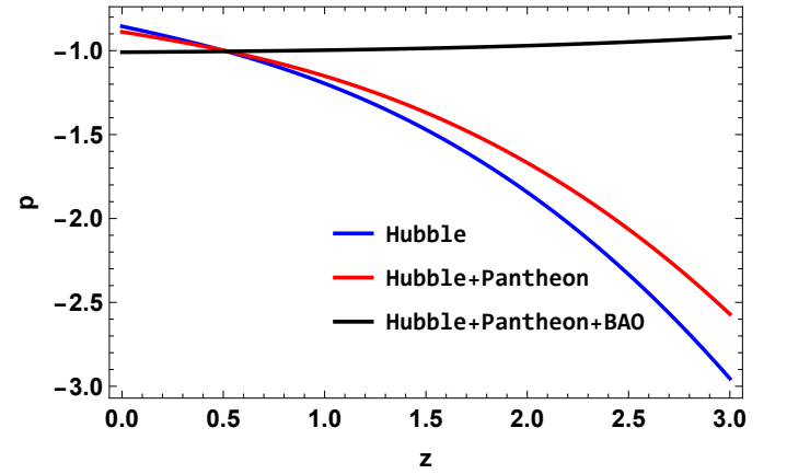
FIG. 9. The behavior of the pressure p vs. redshift z .
