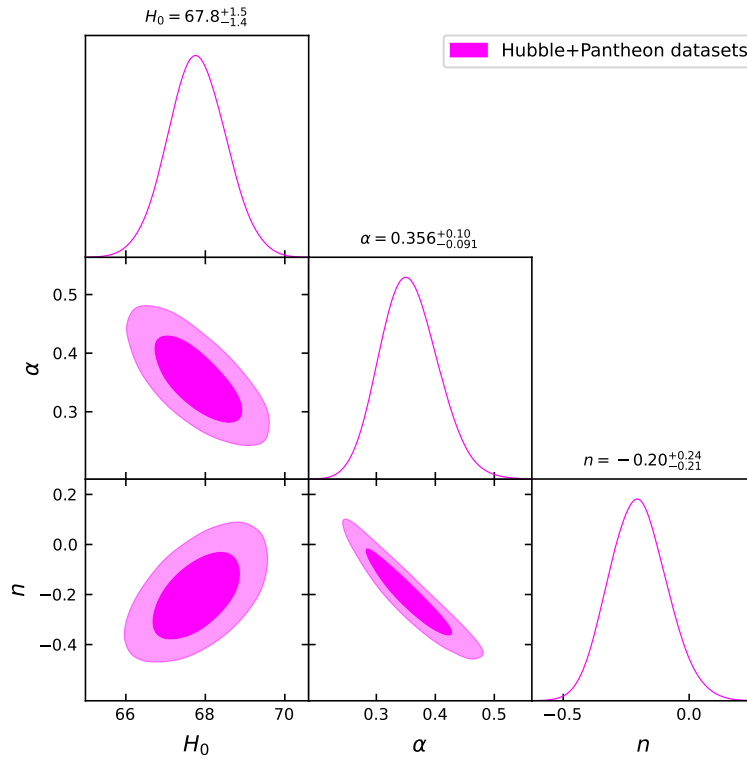
FIG. 4. The confidence curves at 1 - \sigma and 2 - \sigma and posterior distributions for the model parameters using Hubble+Pantheon datasets. The dark pink shaded areas represent the 1 - \sigma confidence level (CL), while the light pink shaded areas represent the 2 - \sigma CL. The parameter constraint values are also presented at the 1 - \sigma CL.
