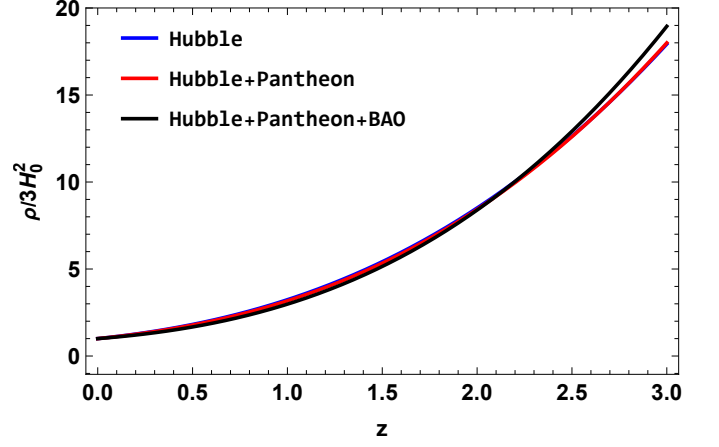
FIG. 8. The behavior of the density parameter \rho vs. redshift z .
