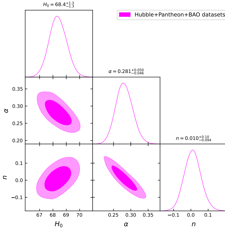
FIG. 5. The confidence curves at 1 - \sigma and 2 - \sigma and posterior distributions for the model parameters using Hubble+Pantheon+BAO datasets. The dark pink shaded areas represent the 1 - \sigma confidence level (CL), while the light pink shaded areas represent the 2 - \sigma CL. The parameter constraint values are also presented at the 1 - \sigma CL.
