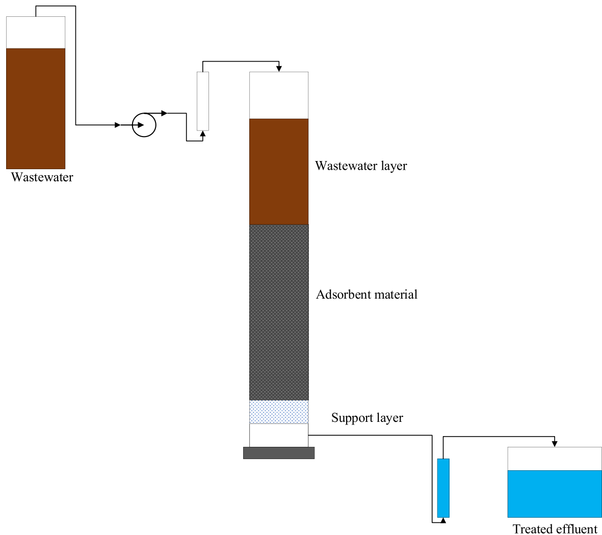
Fig. 1. Filtration setup.
