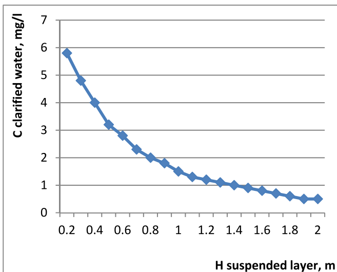
Fig. 6. Graph of dependence of ( C_{cl} ) on ( H_{sus,l} ).
