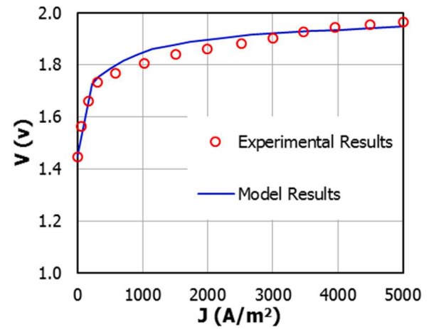
Fig. 5. Comparison of experimental data and numerical modeling results for electrolyzer model.
