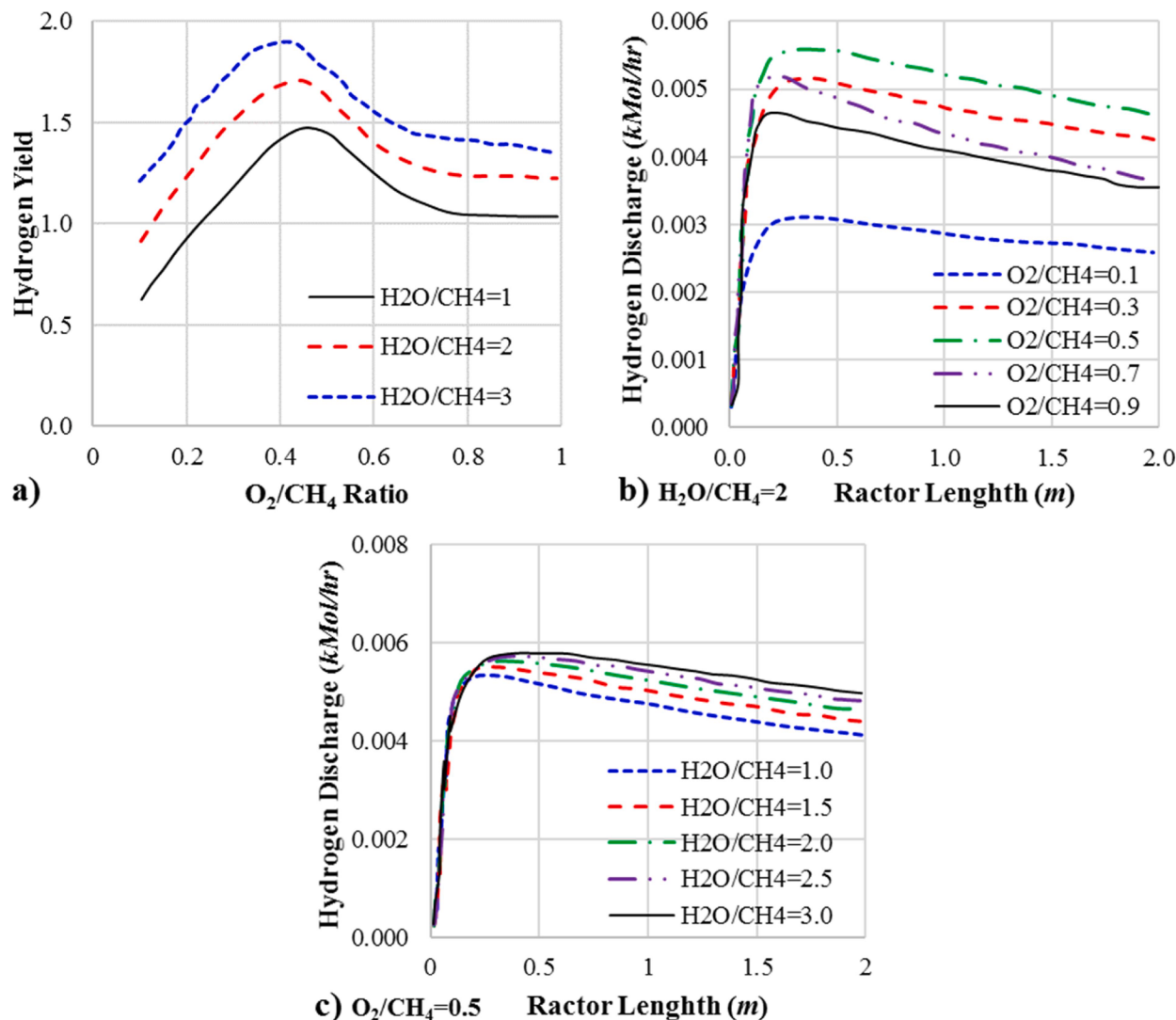
Fig. 3. a. Impact of O_2/CH_4 & H_2O/CH_4 on the hydrogen yield in the carbon dioxide membrane reactor b. Impact of O_2/CH_4 on the hydrogen mol discharge in the carbon dioxide membrane reactor c. Impact of H_2O/CH_4 on the hydrogen mol discharge in the carbon dioxide membrane reactor.
