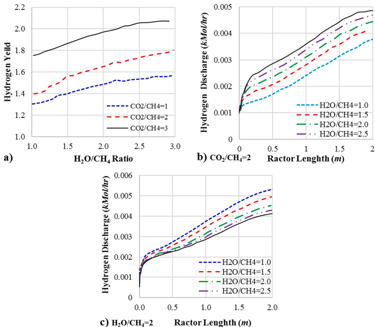
Fig. 1. a. Impact of H 2 O/CH 4 & CO 2 /CH 4 on the hydrogen yield in the oxygen membrane reactor b. Impact of H 2 O/CH 4 on the hydrogen mol discharge in the oxygen membrane reactor c. Impact of CO 2 /CH 4 on the hydrogen mol discharge in the oxygen membrane reactor.
