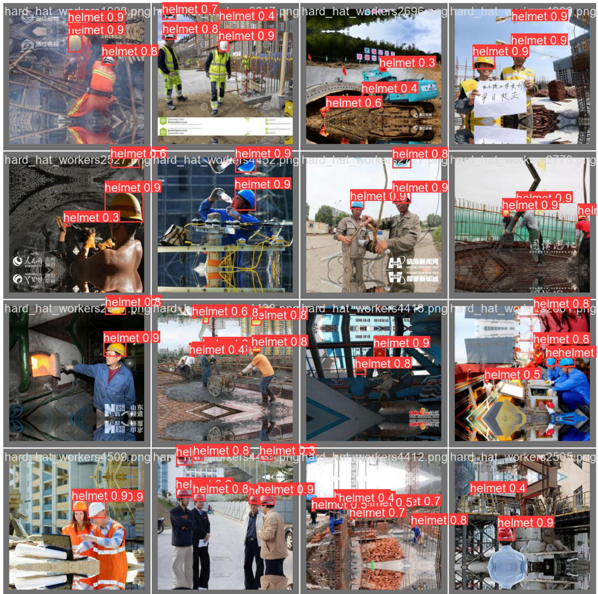
Figure 9. Several satisfactory results of the YOLOv8m/SHELK5K.
