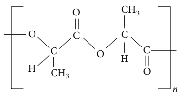
FIGURE 1: Polylactic acid.
