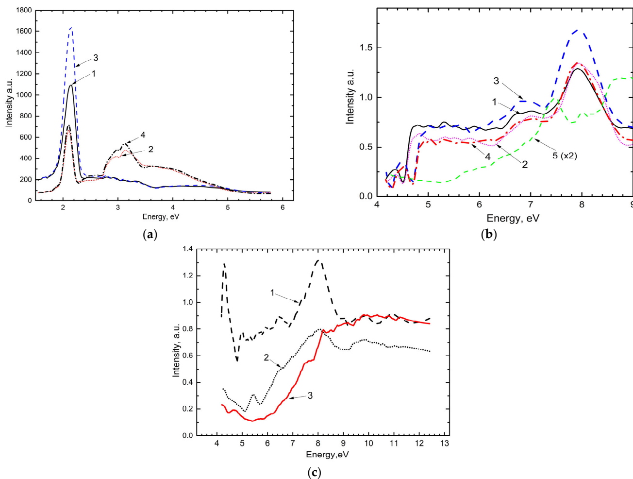
Figure 6. Emission and excitation spectra of the samples. \text{Ca}_2\text{P}_2\text{O}_7 (a) phosphor when excited by photons of 8.26 eV (1—at 300 K; 2—at 15 K) and when excited by photons of 7.75 eV (3—at 300 K; 4—at 15 K). \text{Ca}_2\text{P}_2\text{O}_7 - \text{Mn} (b) for the emission band at 2.0 eV: 1—at 300 K; 2—at 15 K; for the emission band at 2.1 eV: 3—at 300 K; 4—at 15 K; and for the emission band at 2.95 eV: 5—at 15 K. \text{BaSO}_4 - \text{Dy} (c) in the VUV region for emission bands: 1—2.16 eV; 2—2.56 eV; 3—3.1 eV.
