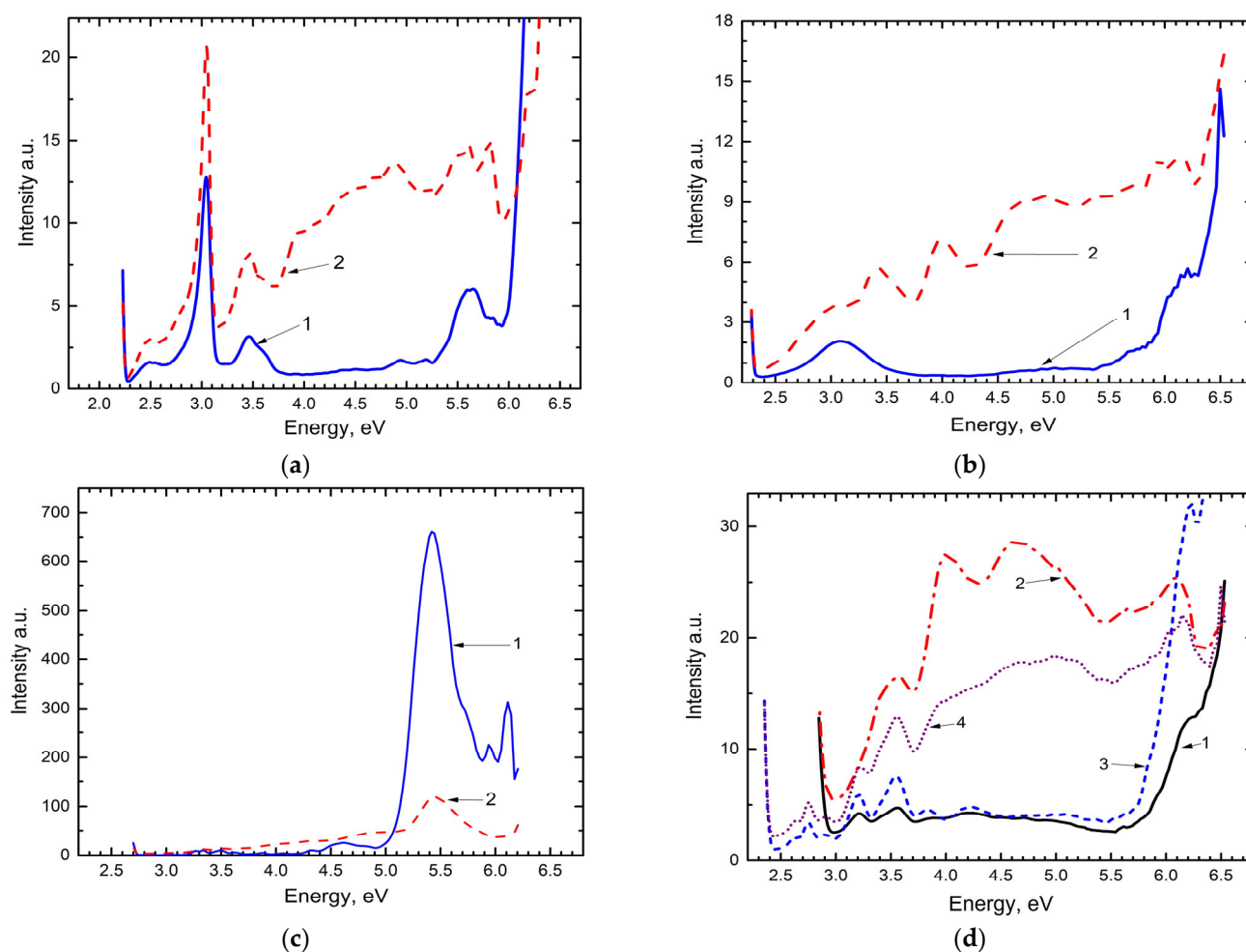
Figure 4. Excitation spectra of intracenter emission. \text{Ca}_2\text{P}_2\text{O}_7 - \text{Mn} (a) emission for the 2.06 eV band (1—at 300 K; 2—at 77 K). \text{Ca}_3(\text{PO}_4)_2 - \text{Mn} (b) emission for the 2.06 eV band (1—at 300 K; 2—at 77 K). \text{Ca}_2\text{P}_2\text{O}_7 - \text{Tb} (c) for the 2.5 eV emission band (curves 1, 2) at 300 K and 77 K. \text{BaSO}_4 - \text{Dy} (d) for the emission bands at 2.56 eV (curves 1, 2) and 2.16 eV (curves 3, 4) at 77 K and 300 K.
