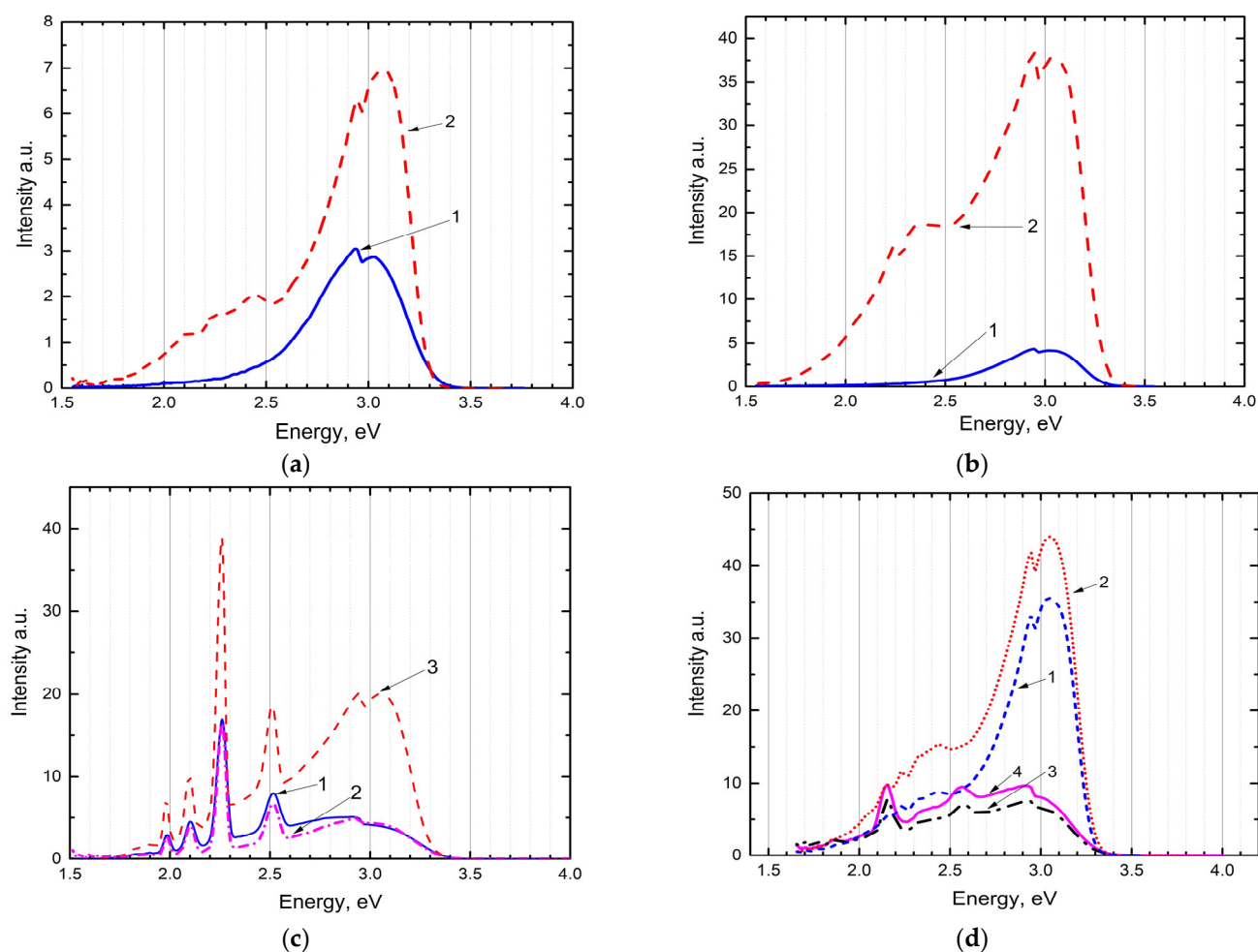
Figure 5. Emission spectra of the phosphor. \text{Ca}_2\text{P}_2\text{O}_7 - \text{Mn} (a) when excited by photons with energies of 3.95–4.0 eV at 300 K and 77 K (curves 1, 2). \text{Ca}_3(\text{PO}_4)_2 - \text{Mn} (b) when excited by photons with an energy of 3.9–4.0 eV at 300 K (curves 1) and 77 K (curves 2). \text{Ca}_2\text{P}_2\text{O}_7 - \text{Tb} (c) when excited by photons with an energy of 3.9 eV: 1—at 300 K; 3—at 77 K; and 4.4 eV: 2—at 300 K. \text{BaSO}_4 - \text{Dy} (d) when excited by photons with an energy of 3.95–4.0 eV (curves 3, 4) and 4.5–4.6 eV at 300 K and 77 K, respectively (curves 1, 2).
