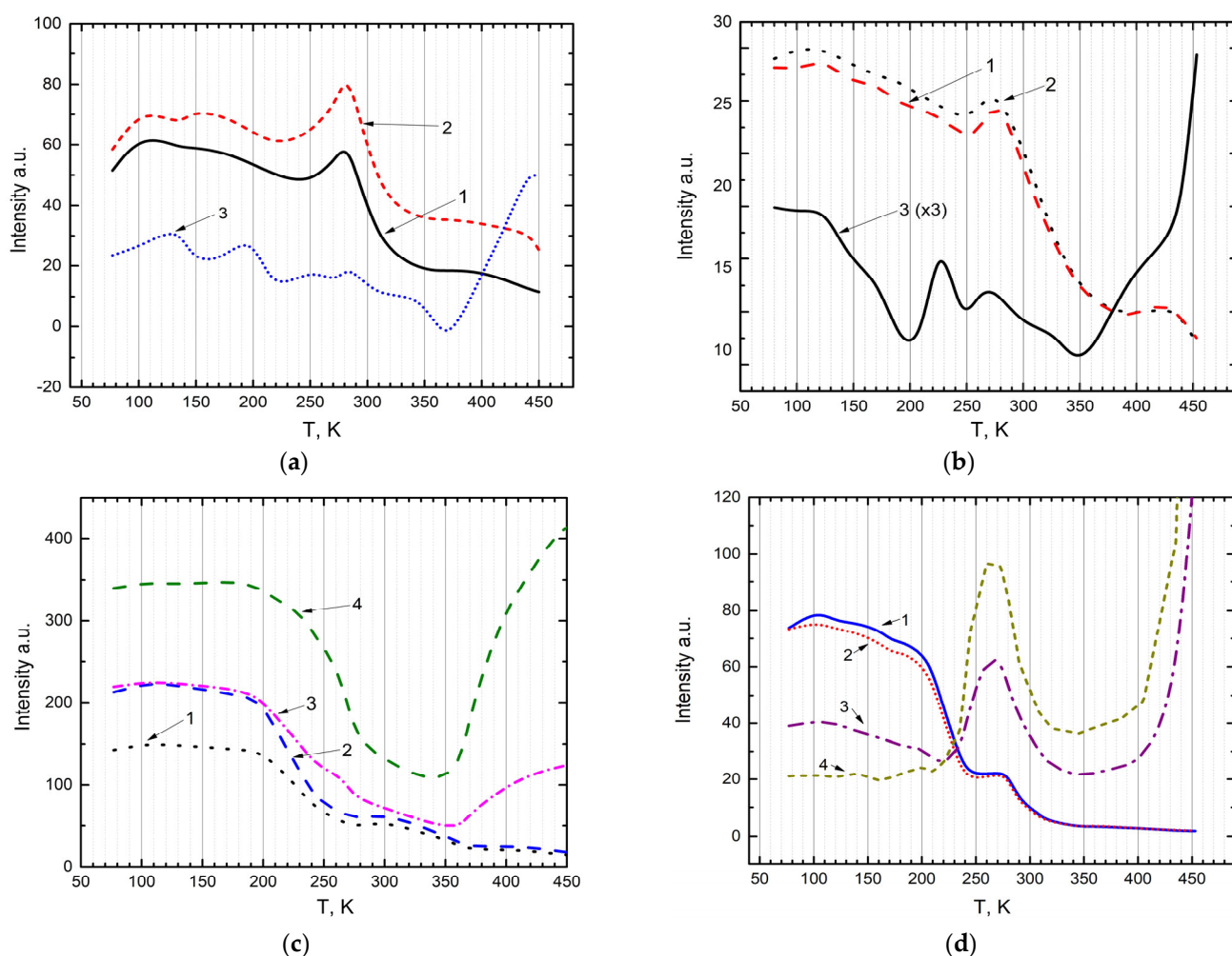
Figure 7. Temperature dependence of the emission. \text{Ca}_2\text{P}_2\text{O}_7 - \text{Mn} (a): 1—at 2.95 eV; 2—at 3.1 eV; 3—at 2.06 eV. \text{Ca}_3(\text{PO}_4)_2 - \text{Mn} (b): 1—at 2.95 eV; 2—at 3.1 eV; 3—at 2.06 eV (curve 3, magnified three times). \text{Ca}_2\text{P}_2\text{O}_7 - \text{Tb} (c) for the emission bands: (1) 3.1 eV; (2) 2.92 eV; (3) 2.51 eV; (4) 2.25 eV. \text{BaSO}_4 - \text{Dy} (d) for the emission bands: (1) 3.1 eV; (2) 2.95 eV; (3) 2.56 eV; (4) 2.16 eV.
