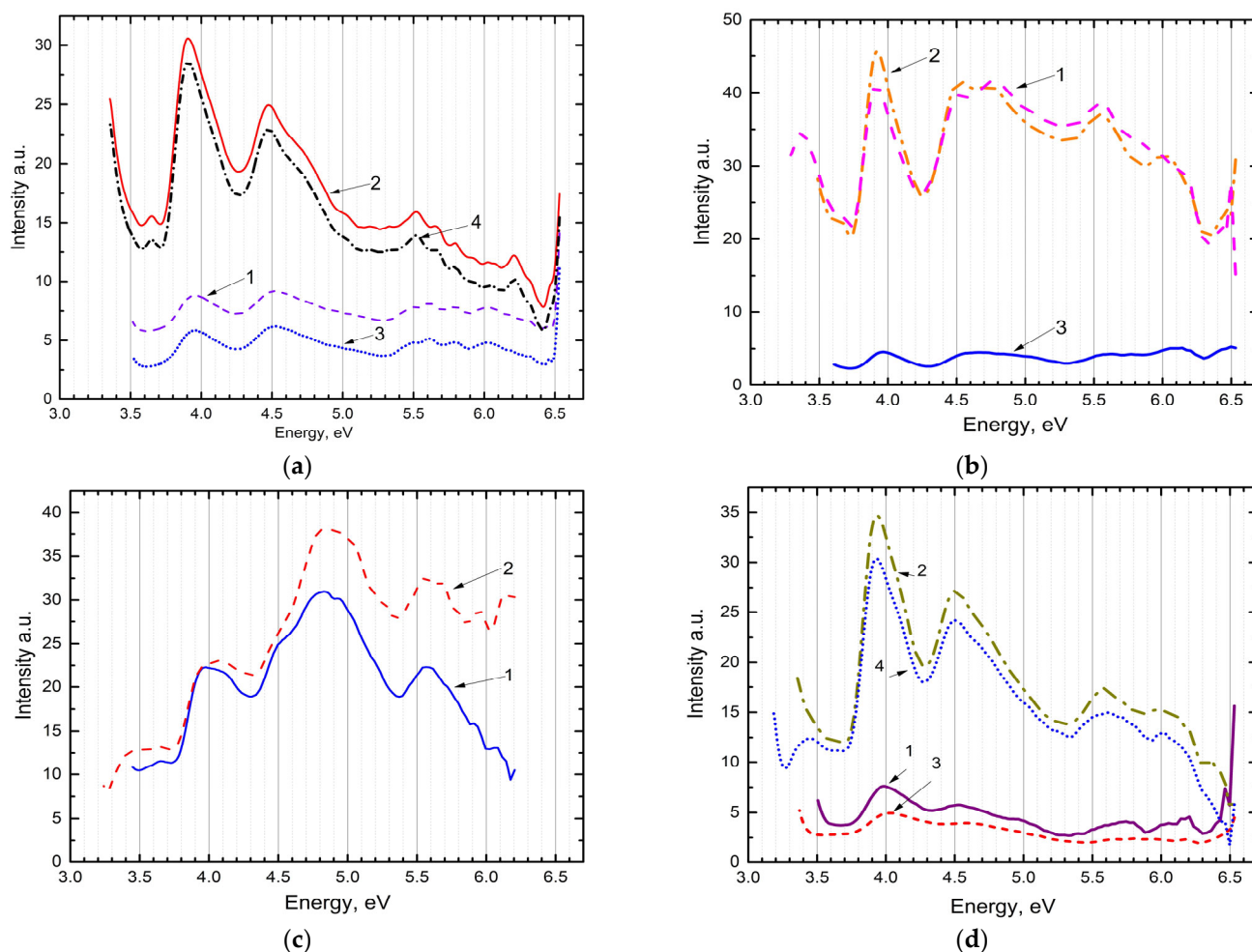
Figure 3. Excitation spectra of pre-irradiated phosphor. Ca_2P_2O_7 - Mn (a) 1—for the emission band at 2.92 eV at 300 K; 2—for the emission band at 2.92 eV at 77 K; 3—for the emission band at 3.06 eV at 300 K; 4—for the emission band at 3.06 eV at 77 K. Ca_3(PO_4)_2 - Mn (b) 1—for the emission band at 2.92 eV at 77 K; 2—for the emission band at 3.06 eV at 77 K; 3—for the emission band at 3.06 eV at 300 K. Ca_2P_2O_7 - Tb (c) 1—for the emission band at 3.1 eV at 77 K; 2—for the emission band at 2.93 eV at 77 K. BaSO_4 - Dy (d) for the emission band at 2.95 eV at 300 K (curve 1), at 77 K (curve 2), and for the band at 3.1 eV at 300 K (curve 3) and at 77 K (curve 4).
