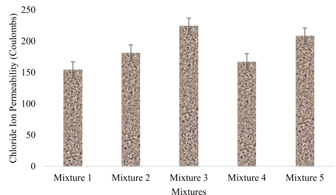
Fig. 5. Chloride Ion Permeability results.
