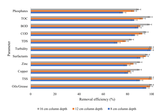
Fig. 3. Removal efficiencies from different parameters.
