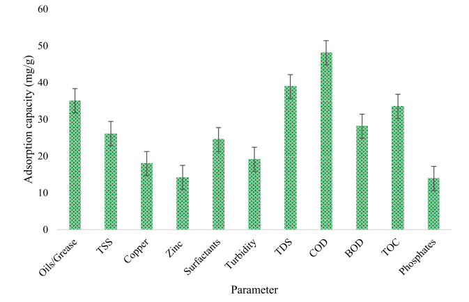
Fig. 4. Adsorption capacities from different parameters.
