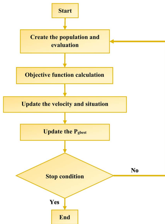
Figure 1. PSO flowchart.
