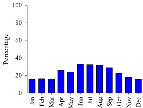
Figure 4. The attain energy receive in different mouths by optimal angel using isotropic model.
