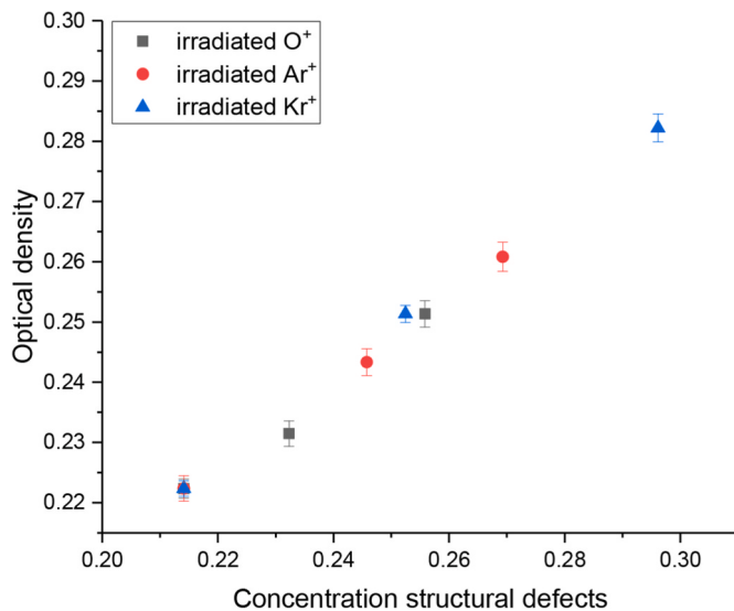
Fig. 3. Results of comparative analysis of the connection between the change in optical density and the concentration of structural defects in ZnO/CoZn nanostructures caused by heavy ion irradiation at irradiation fluence variation.
