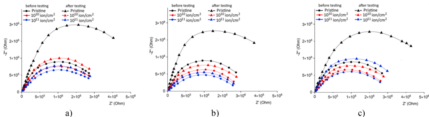
Fig. 8. Results of constructing Nyquist plots Z'' ( Z' ) for the studied samples in comparison before and after testing, reflecting the resistance growth caused by the degradation of the anode material associated with the lithiation and oxidation processes: a) in case of modification by O^+ ions; b) in case of modification by Ar^+ ions; c) in case of modification by Kr^+ ions.
