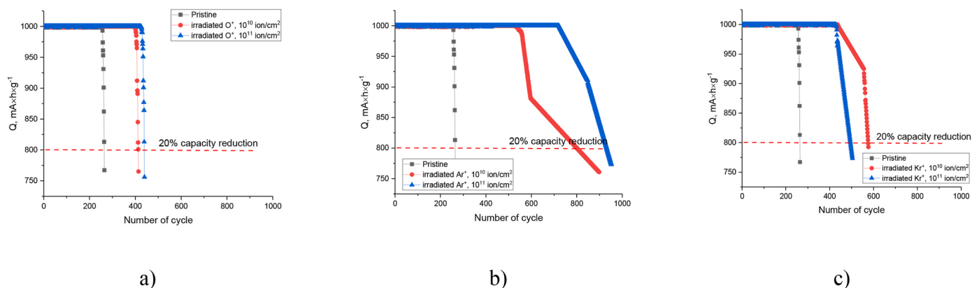
Fig. 5. Results of resource cyclic tests of the studied ZnO/CoZn nanostructures as anode materials, reflecting the change in the efficiency of their use as anode materials (The dotted line indicates the capacity value, which is 80 % of the nominal value, chosen as a value characteristic of the degradation stage of nanostructures.): a) in case of modification by O^+ ions; b) in case of modification by Ar^+ ions; c) in case of modification by Kr^+ ions.
