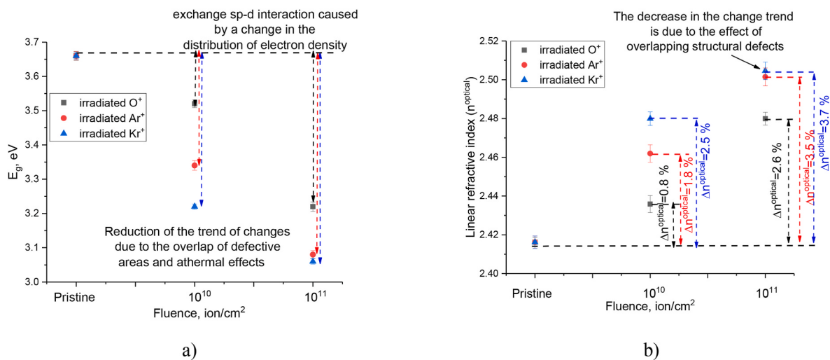
Fig. 2. Results of evaluation of optical and electronic properties of ZnO/CoZn nanostructures: a) Results of changes in the E_g value of the studied ZnO/CoZn nanostructures before and after ion modification; b) Results of comparative analysis of changes in the linear refractive index for ZnO/CoZn nanostructures depending on the type of ions and irradiation fluence.
