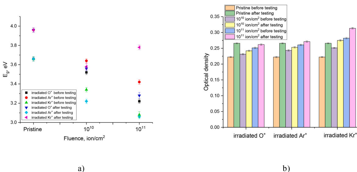
Fig. 9. a) Results of alterations in the E_g value for the studied ZnO/CoZn nanostructures before and after resource tests as anode materials; b) Results of alterations in the optical density value for ZnO/CoZn nanostructures before and after resource tests as anode materials.
