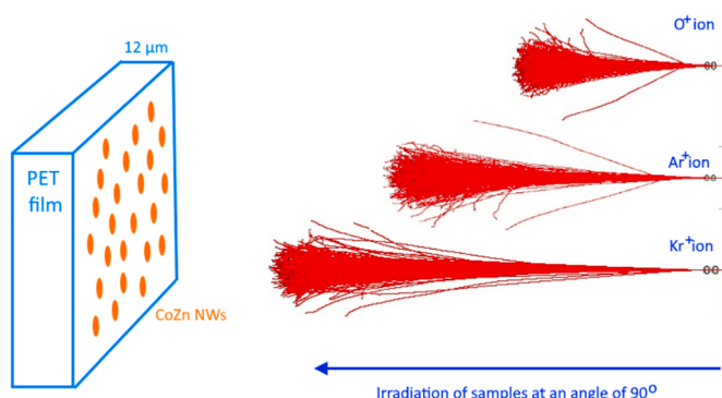
Fig. 1. Scheme of conducting experiments on irradiation.
