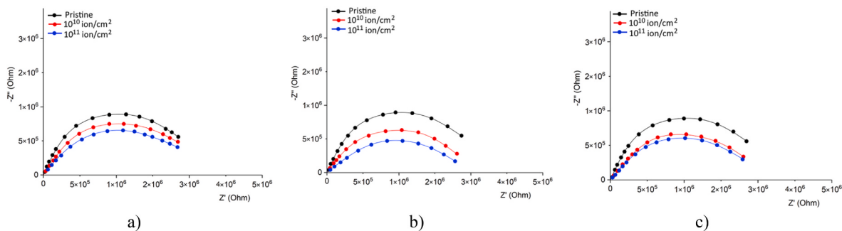
Fig. 4. Results of constructing Nyquist plots Z'' ( Z' ) for the studied samples of ZnO/CoZn nanostructures depending on the type of ion exposure: a) in case of modification by O^+ ions; b) in case of modification by Ar^+ ions; c) in case of modification by Kr^+ ions.
