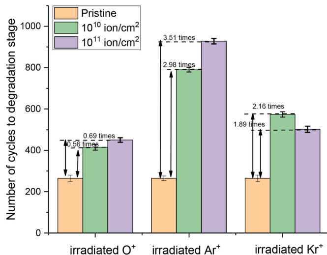
Fig. 6. Comparative diagram reflecting the number of cycles of resource tests of ZnO/CoZn nanostructures as anode materials, after which a decrease in capacity below 80 % of the nominal value is observed, the value of which is the limit of the operating mode (the dotted lines reflect the values of the increase in the number of test cycles for modified nanostructures in comparison with unmodified ZnO/CoZn nanostructures).
