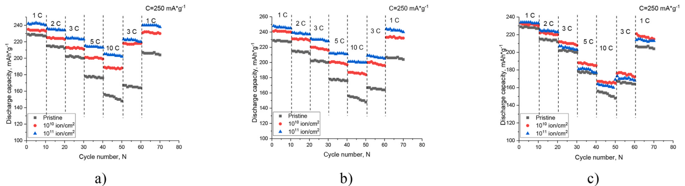
Fig. 7. Results of tests of ZnO/CoZn nanostructures as anode materials at charging rate variation: a) in case of modification of ZnO/CoZn nanostructures by \text{O}^+ ions; b) in case of modification by \text{Ar}^+ ions; c) in case of modification by \text{Kr}^+ ions.
