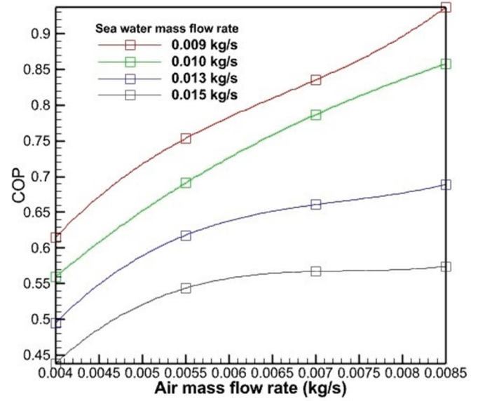
Fig. 6. COP system in different AMFRs.
