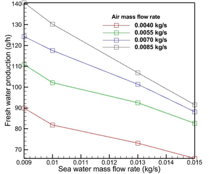
Fig. 7. The MFR of fresh water produced in different SWMFRs.
