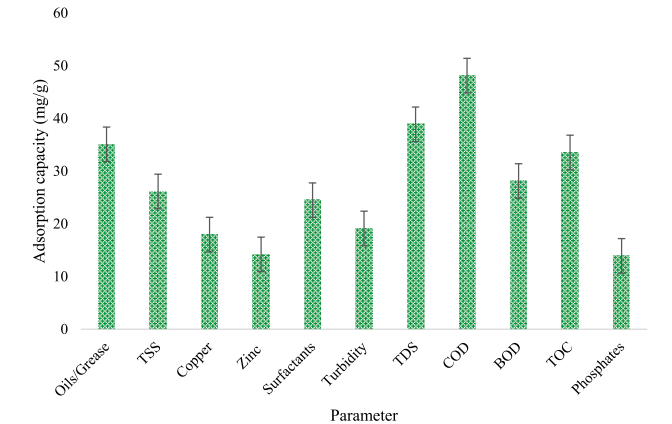
Fig. 4. Adsorption capacities from different parameters.
