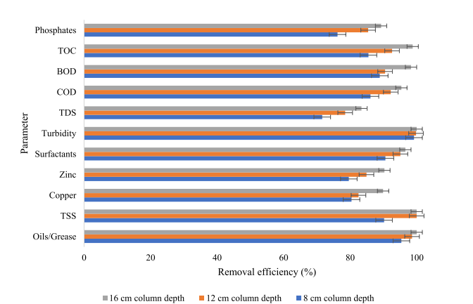
Fig. 3. Removal efficiencies from different parameters.
