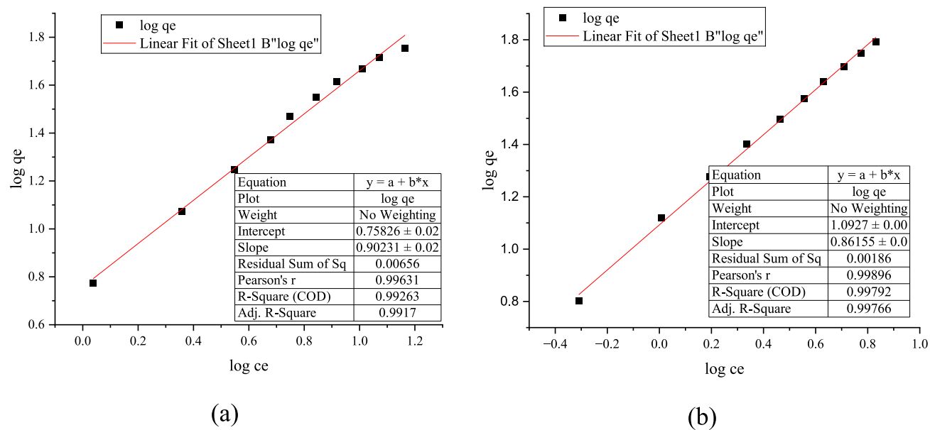
Fig. 4. Freundlich adsorption isotherm (a) without biofilm (b) with biofilm.
