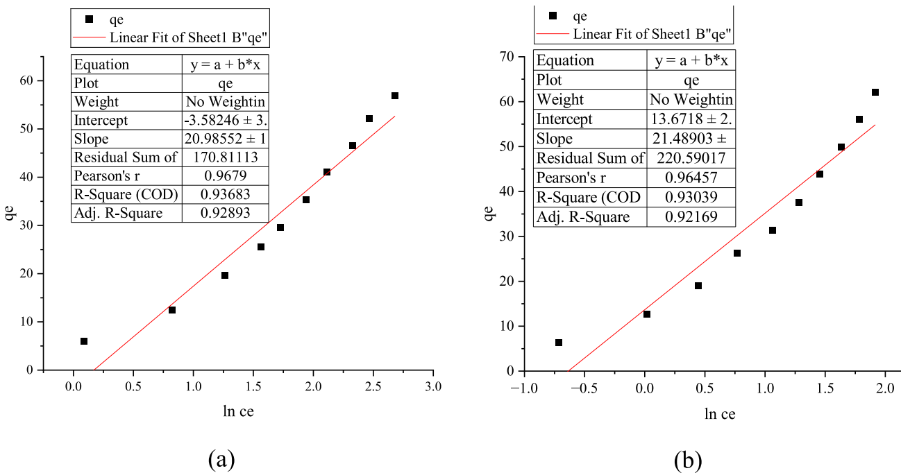
Fig. 5. Temkin adsorption isotherm (a) without biofilm (b) with biofilm.
