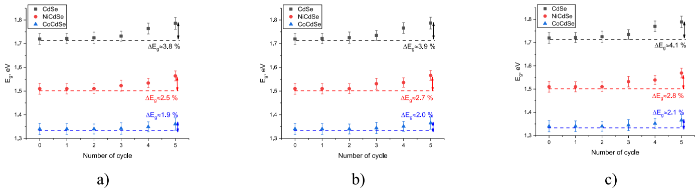
Fig. 6. Results of changes in the band gap value of the studied films contingent upon the number of test cycles: a) during iron adsorption; b) during manganese adsorption; c) during arsenic adsorption.
