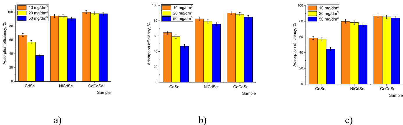
Fig. 4. Evaluation results of the efficiency of purification of model solutions using thin films of different composition as catalysts: a) during iron adsorption; b) during manganese adsorption; c) during arsenic adsorption.
