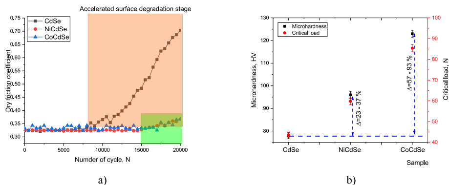
Fig. 2. Results of measurements of strength parameters of the studied films: a) results of tribological tests (The highlighted areas indicate the main changes in the dry friction coefficient in the case of the original CdSe films (orange area) and modified ones (green area)); b) results of measurements of hardness and adhesive strength. (For interpretation of the references to colour in this figure legend, the reader is referred to the Web version of this article.)
