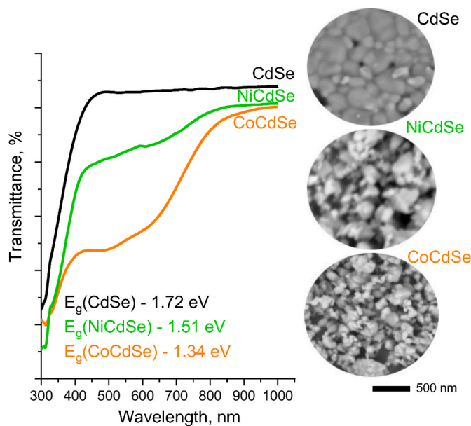
Fig. 1. Results of optical transmission spectra of the studied films contingent upon the dopant type, and the insets show the results of morphological features that determine changes in transmission capacity in the visible light region.
