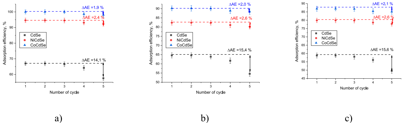
Fig. 5. Assessment results of changes in the adsorption capacity efficiency of thin films with an increase in the number of consecutive test cycles: a) during iron adsorption; b) during manganese adsorption; c) during arsenic adsorption.
