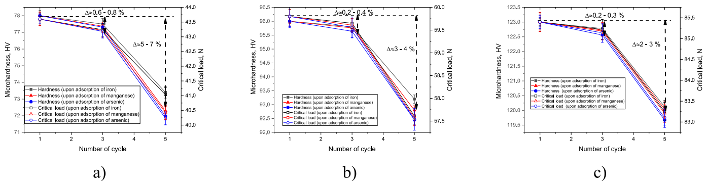
Fig. 7. Results of changes in the strength parameters of the studied films in the case of cyclic tests for maintaining the efficiency of catalytic activity: a) CdSe films; b) NiCdSe films; c) CoCdSe films.
