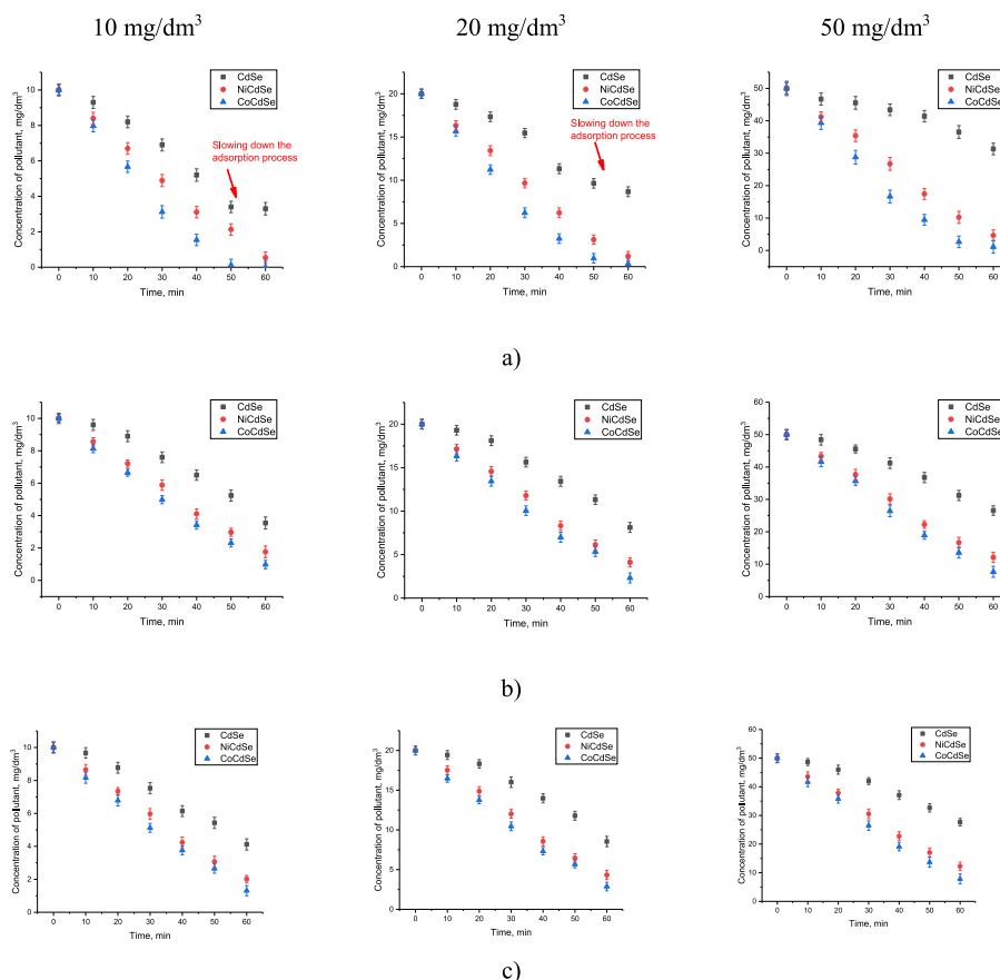
Fig. 3. Assessment results of the pollutant concentration change in a model solution with variation in pollutant concentration in the case of: a) iron adsorption; b) manganese adsorption; c) arsenic adsorption.
