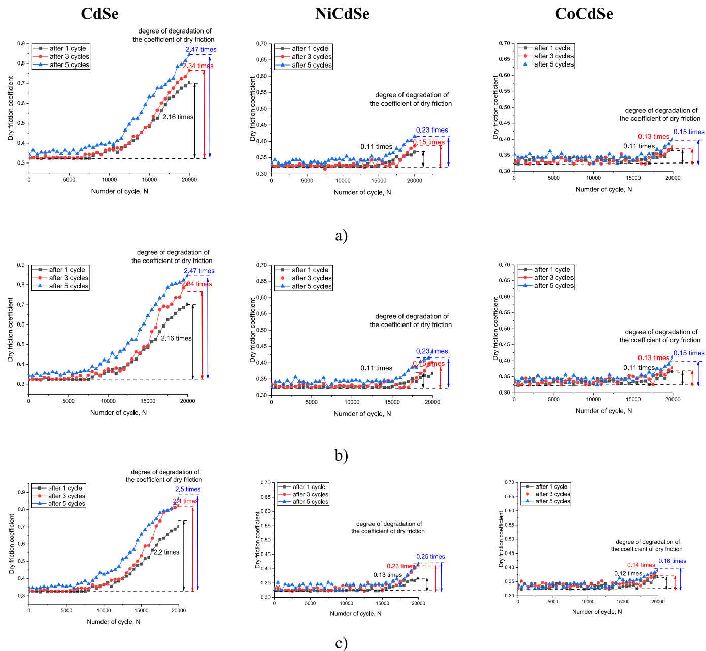
Fig. 8. Results of tribological tests of the studied films after cyclic tests for maintaining the efficiency of catalytic activity: a) during iron adsorption; b) during manganese adsorption; c) during arsenic adsorption.
