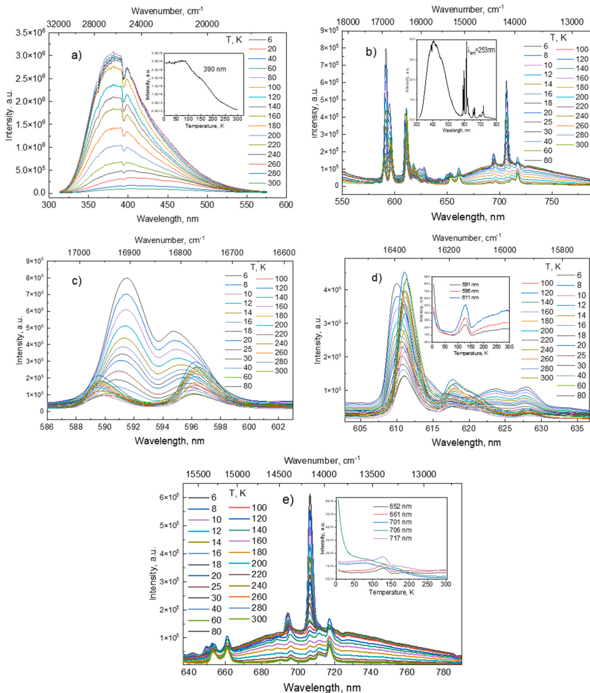
Fig. 6. Temperature dependence of the luminescence of Ga 2 O 3 :Eu ceramics (a) in the 300–575 nm range with the temperature dependence of emission at 390 nm in the inset; (b) in the 550–800 nm range with the luminescence spectrum under 253 nm excitation in the inset; (c) in the 586–602 nm range; (d) in the 605–635 nm range with the emission dependence at 591, 595, and 610 nm in the inset; (e) in the 630–800 nm range with the emission dependence at 652, 661, 701, 706, and 717 nm in the inset; (f) under 260 nm excitation.
