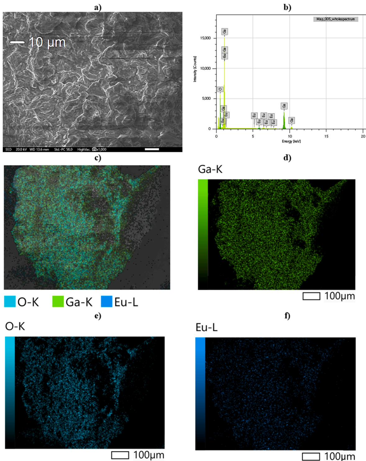
Fig. 2. SEM image (a); EDS spectra (b); Element mapping (c, d, e, f) of \text{Ga}_2\text{O}_3:\text{Eu} ceramic.
