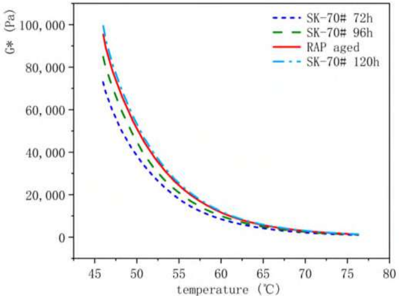
Figure 2. Rheological comparison of TCAOT-aged and conventionally aged asphalt binders — G^*/\delta consistency [7].
