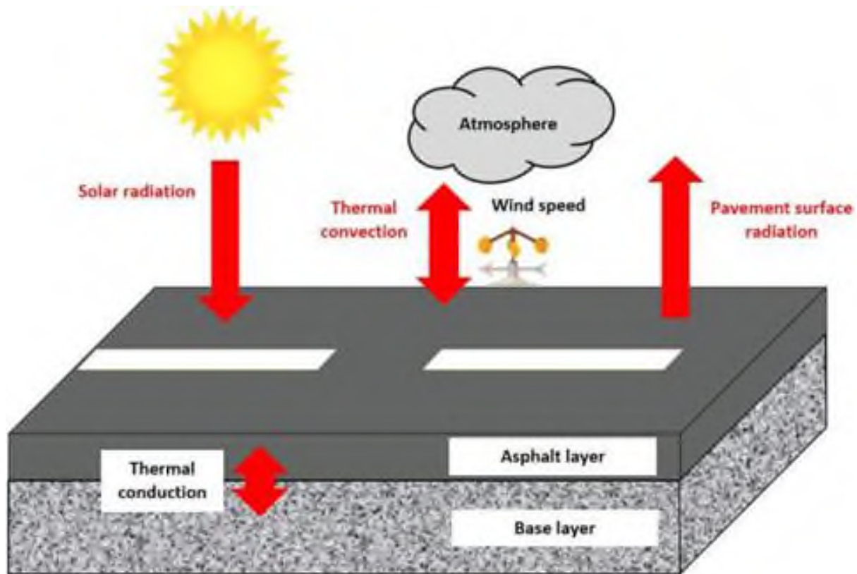
Figure 1. Schematic diagram of heat transfer modes for asphalt pavement [1].
