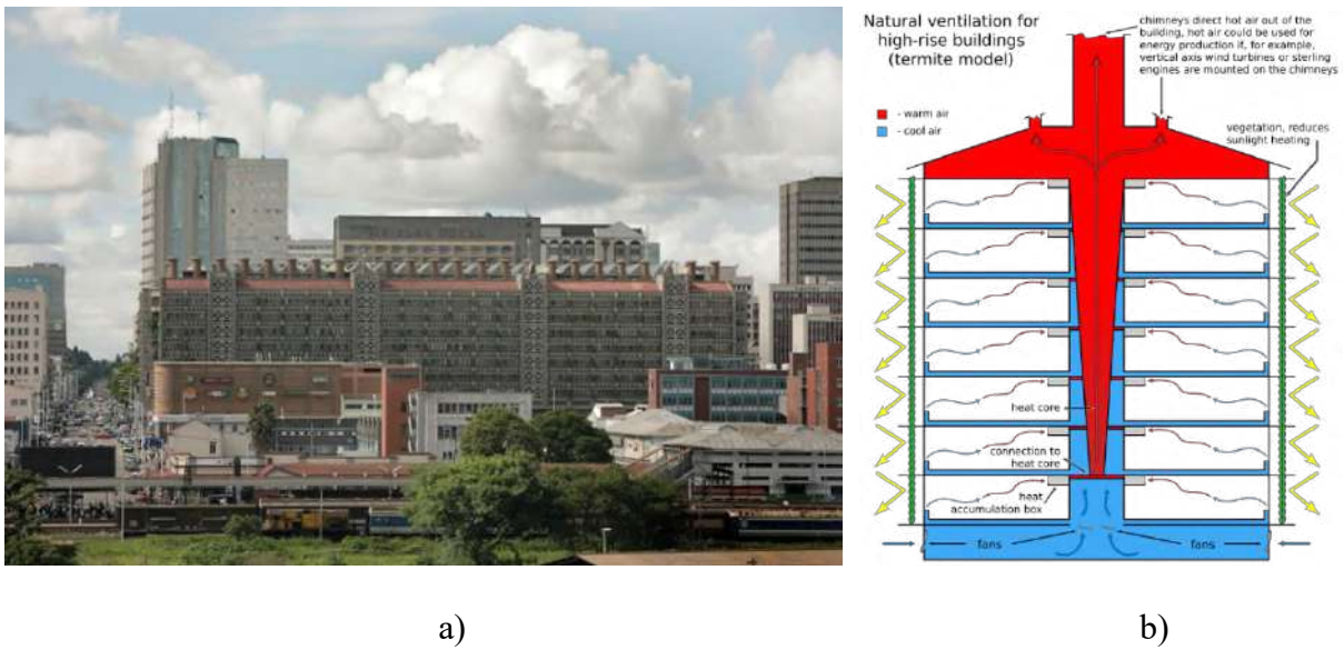
Figure 2. a) The Eastgate Centre in Harare [6]; b) Schematic of the natural ventilation of the building [7].
