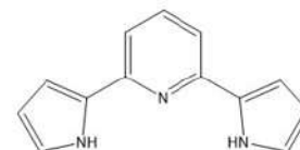
bis-pyrrole – L3
