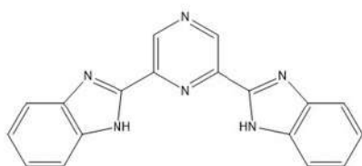
Bzimpyz – L1
