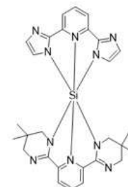
Si-hetero-3 Si(IPI/saturated-bzimpy)
