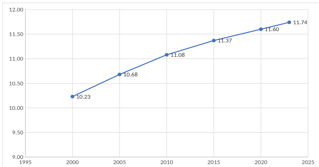
Figure 1. Annual temperature trends in South Kazakhstan, 2000–2023
