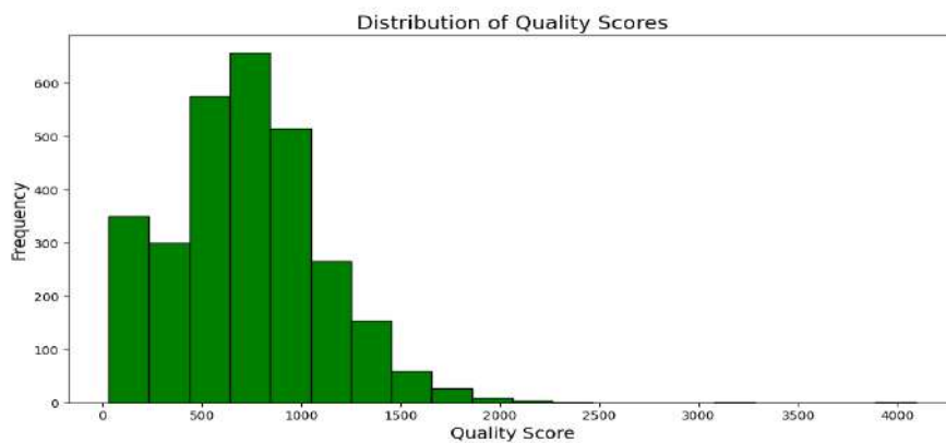
Figure 4 Quality Scores
